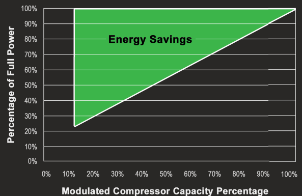
Digital Scroll Linear Power Reduction
